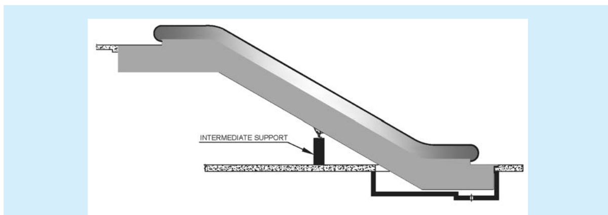
FIG. 11 INTERMEDIATE SUPPORTS
