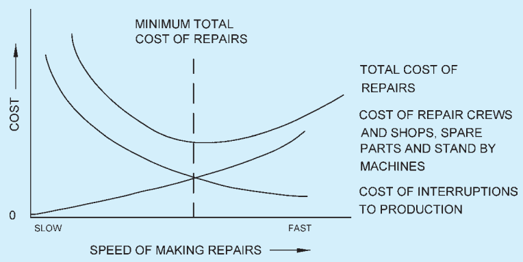
FIG. 4 SPEED OF MAKING REPAIRS
