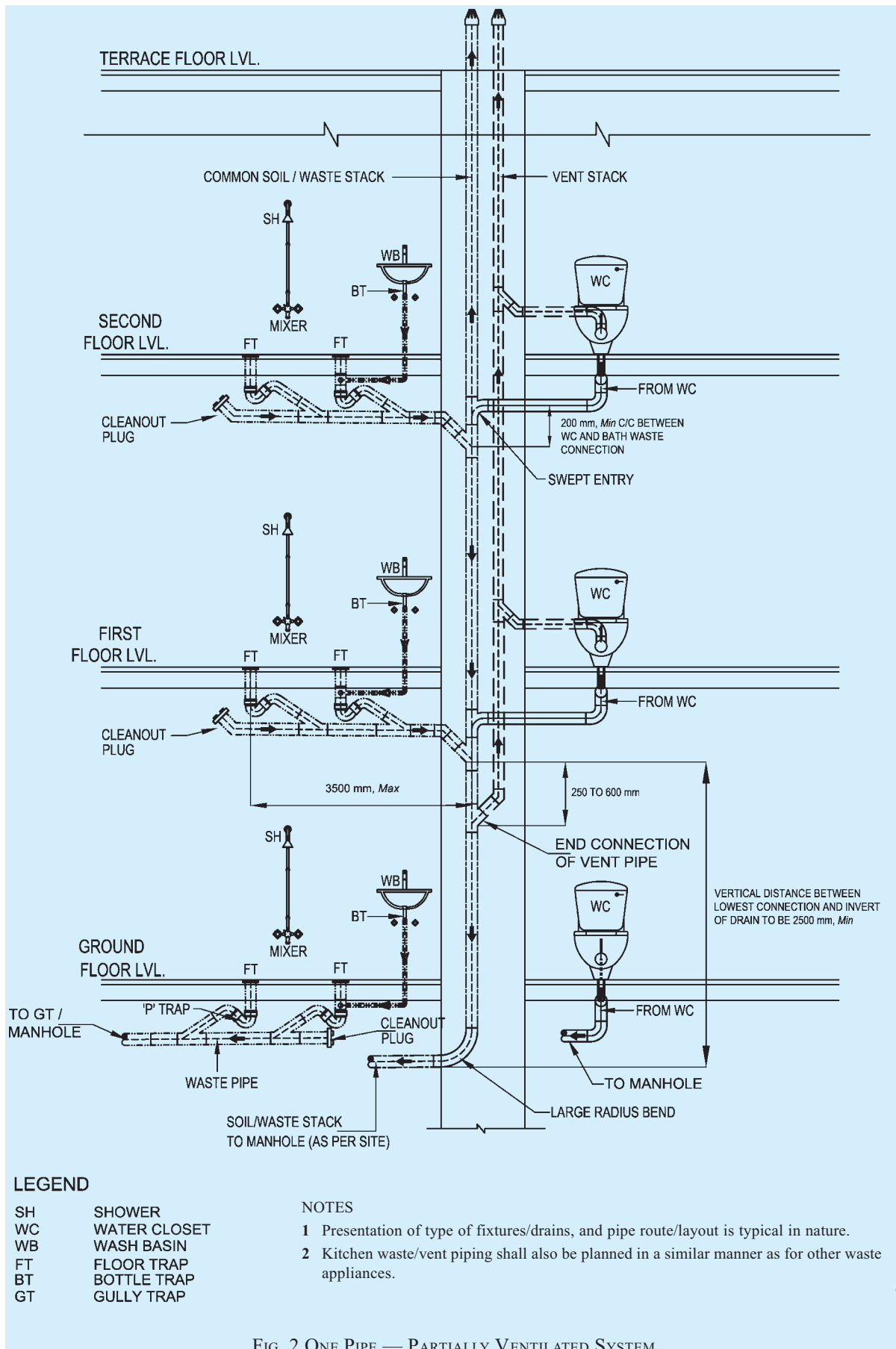
FIG. 2 ONE PIPE — PARTIALLY VENTILATED SYSTEM
