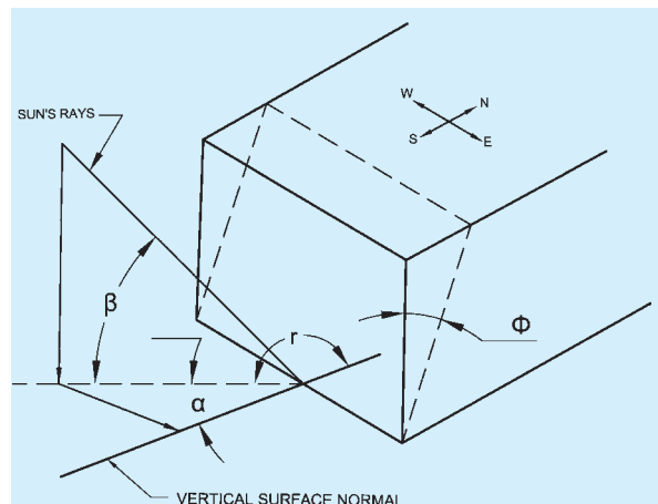
FIG. 12 DEFINITION OF SOLAR ANGLES
