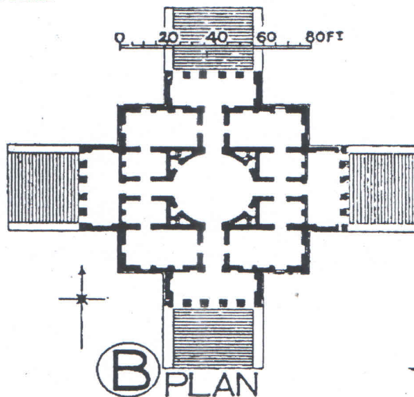
Fig 1. Plan of Villa Capra Vicenza
